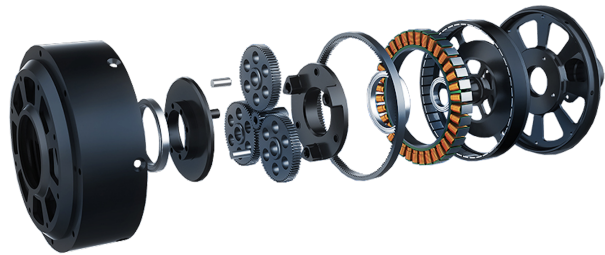
Fig. 2. Exploded view of an open-frame version of T-motor AK80-9 [31].
