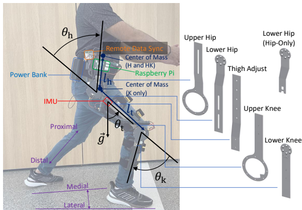
Fig. 4. Left: M-BLUE hip-knee configuration with superimposed joint angle conventions for hip ( \theta_h ) and knee ( \theta_k ) angles, provided by actuator encoders, as well as thigh angle ( \theta_t ) with respect to gravity ( g ), provided by the IMU (red). Thigh ( l_t ) and hip ( l_h ) length parameters, and center of mass for different configurations are shown in dark blue. Other annotated systems include the Raspberry Pi (green), its power source (blue), and a remote data sync board (orange; only required during EMG experiments). A convention for directional vocabulary (purple) is also included for reference. Right: CAD models of the custom sheet metal components used in various configurations.
